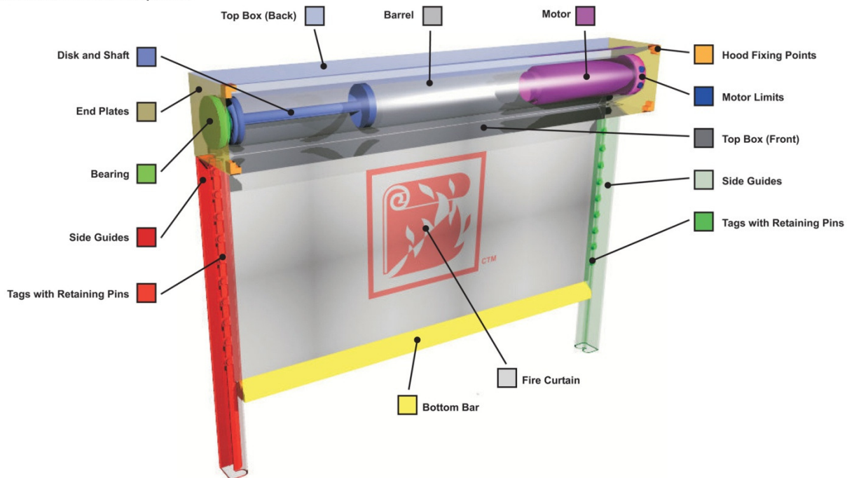
Single Barrel Fire Curtain Explained
