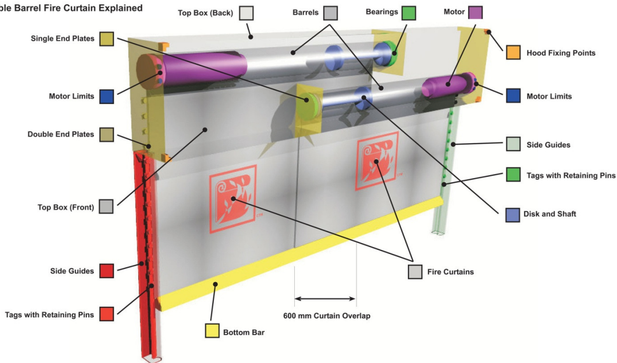
Double Barrel Fire Curtain Explained
